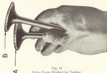
Fig. 11 Valve Faces Marked for Testing "A" face before test—"B" after test. Note broken lines
